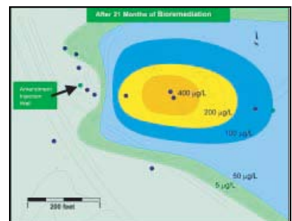
Contaminant plume after 21 months ARD
